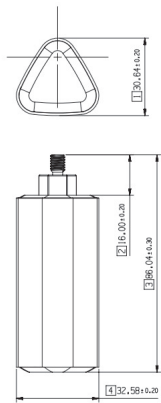
Abmessungen aller Condition-Monitoring OPTIME-Sensoren (3, 5, 5 Ex)
